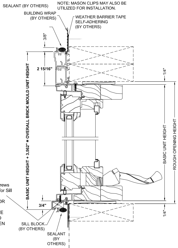
3 1/2" Aluminum Brick Mould L/F Part#
