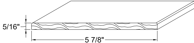
5 7/8" INTERIOR MULL CASING L/F PART NO. 216612
