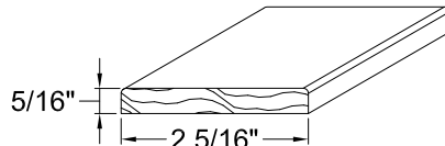
2 5/16" INTERIOR MULL CASING L/F PART NO. 216608
