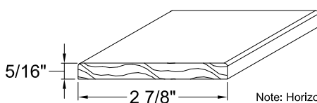
2 7/8" INTERIOR MULL CASING L/F PART NO. 216609
