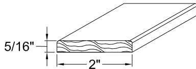
2" INTERIOR MULL CASING L/F PART NO. 216607
