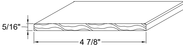
4 7/8" INTERIOR MULL CASING L/F PART NO. 216611
