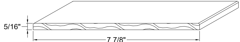
7 7/8" INTERIOR MULL CASING L/F PART NO. 216614
