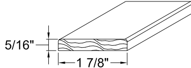
1 7/8" INTERIOR MULL CASING L/F PART NO. 201107
