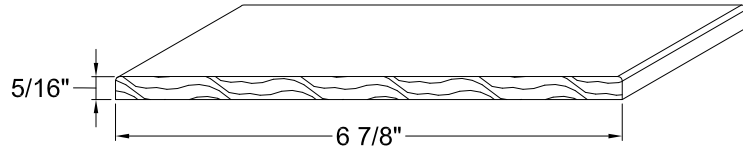
6 7/8" INTERIOR MULL CASING L/F PART NO. 216613
