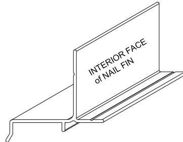
Aluminum Structural Drip Cap Nail Fin
