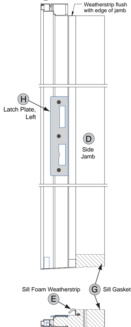
End View of Side Jamb
