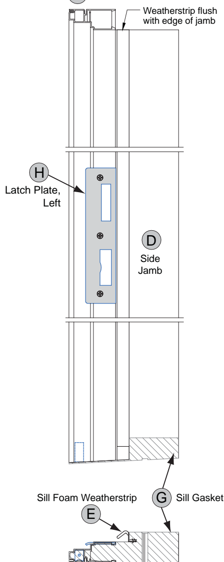
End View of Side Jamb
