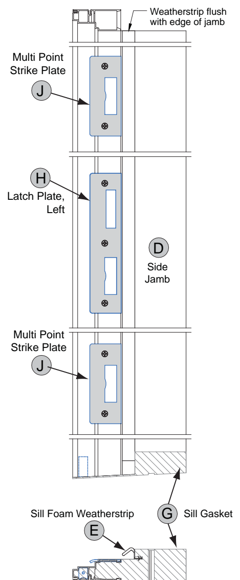
End View of Side Jamb
