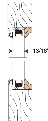
Vertical Section of Panel
