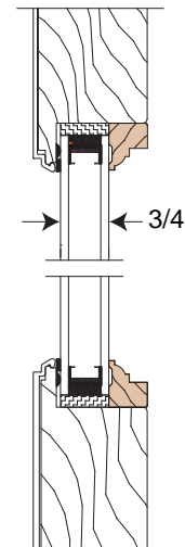
Vertical Section of Panel
