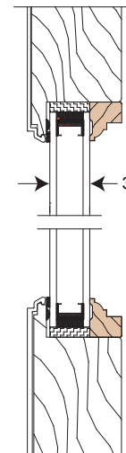
Vertical Section of Panel
