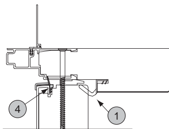
Sidelite / Fixed Panel, Head
