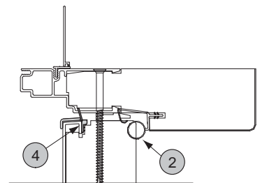
Transom Panel, Head
