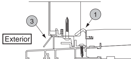
Sidelite / Fixed Panel, Sill
