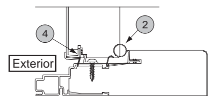
Transom Panel, Sill
