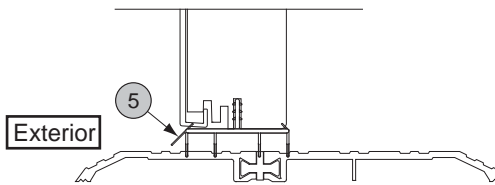
ADA Operating Panel, Sill
